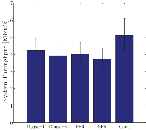
Fig. 5: System throughput
