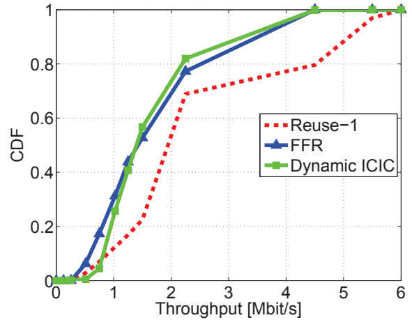
Fig. 3: Throughput cumulative distribution function
